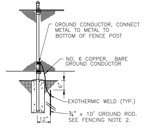
4 FENCE GROUNDING DETAIL C301 SCALE: NTS
