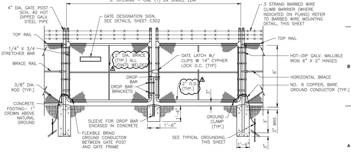
5 SWING GATE DETAIL C301 SCALE: NTS
