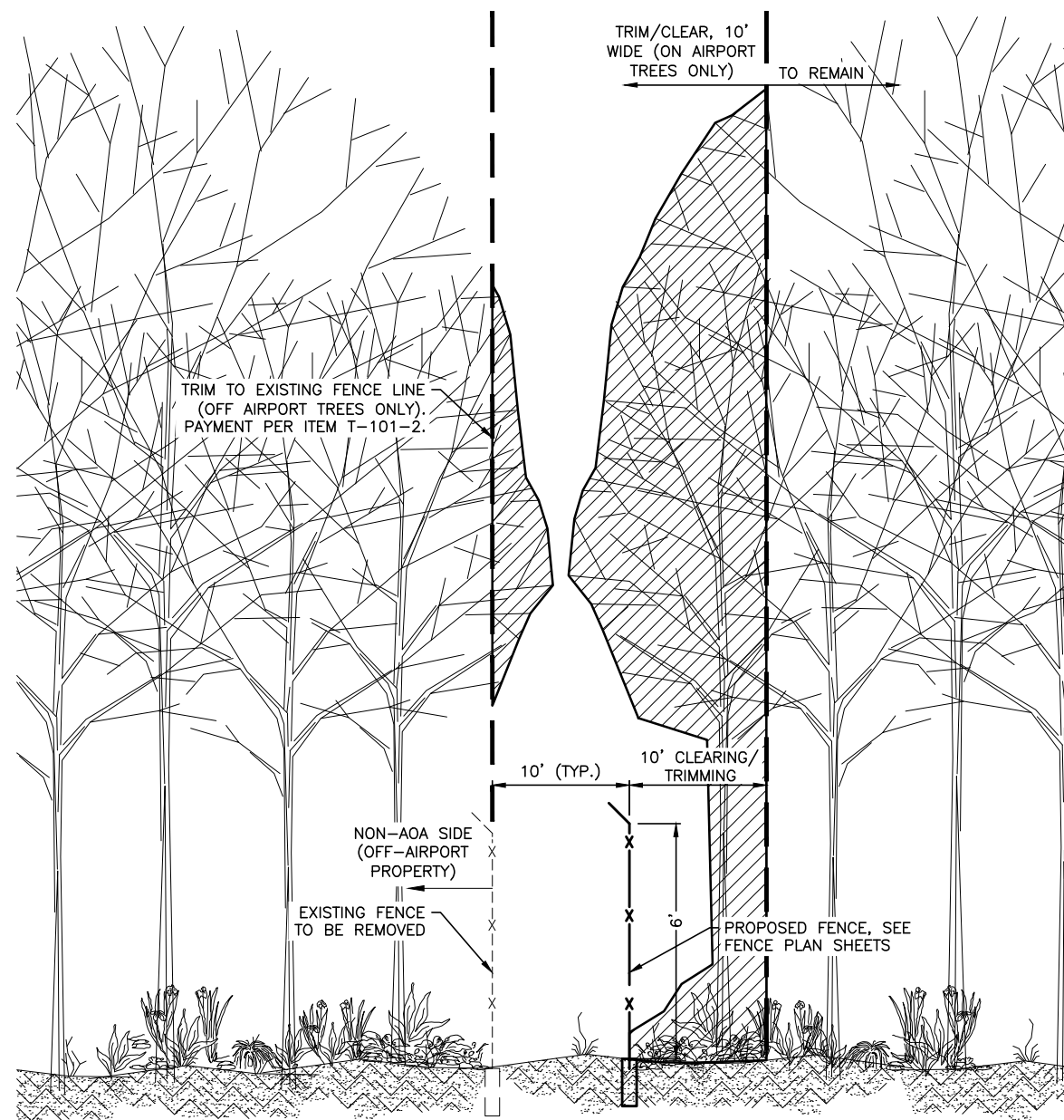
1 TREE CLEARING DETAIL - PCA AREA 1 C301 SCALE: NTS
