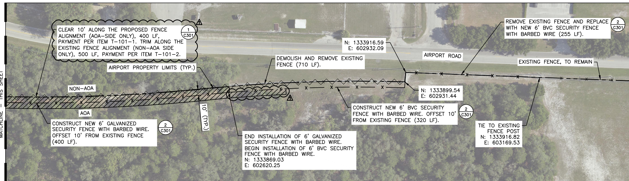
2 FENCE PLAN - AREA 1 C101
