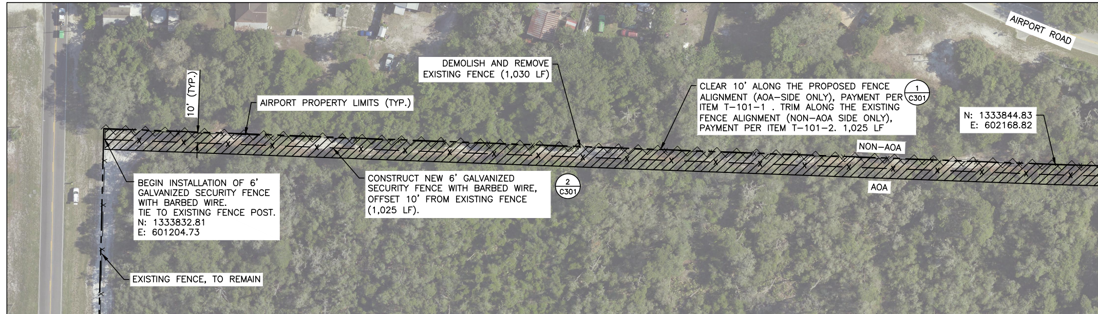
1 FENCE PLAN - AREA 1 C101
