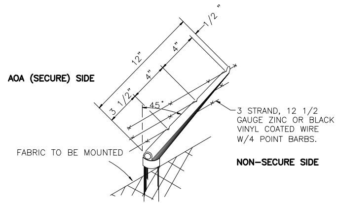
3 BARBED WIRE MOUNTING C301 SCALE: NTS
