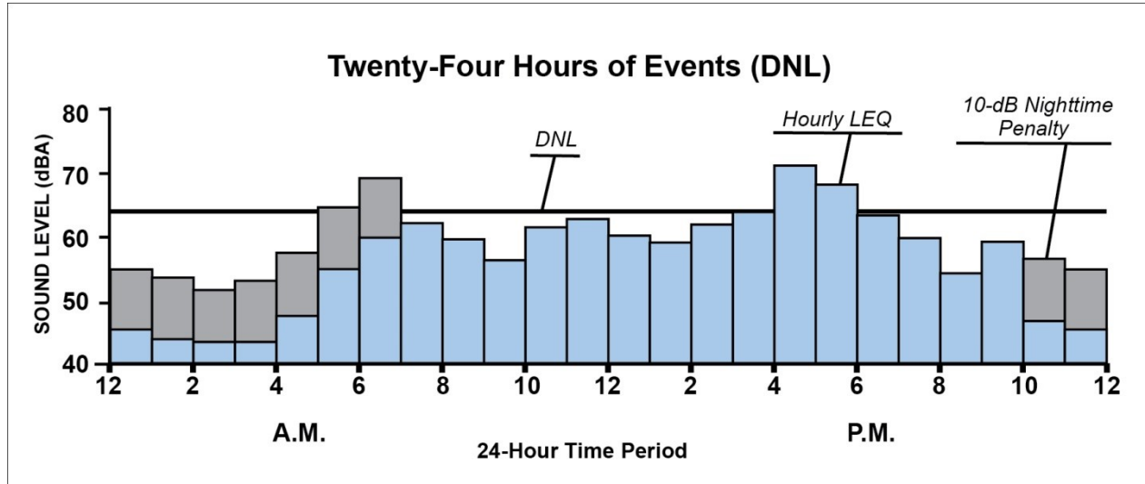
FIGURE D-2 DAY-NIGHT AVERAGE SOUND LEVEL
